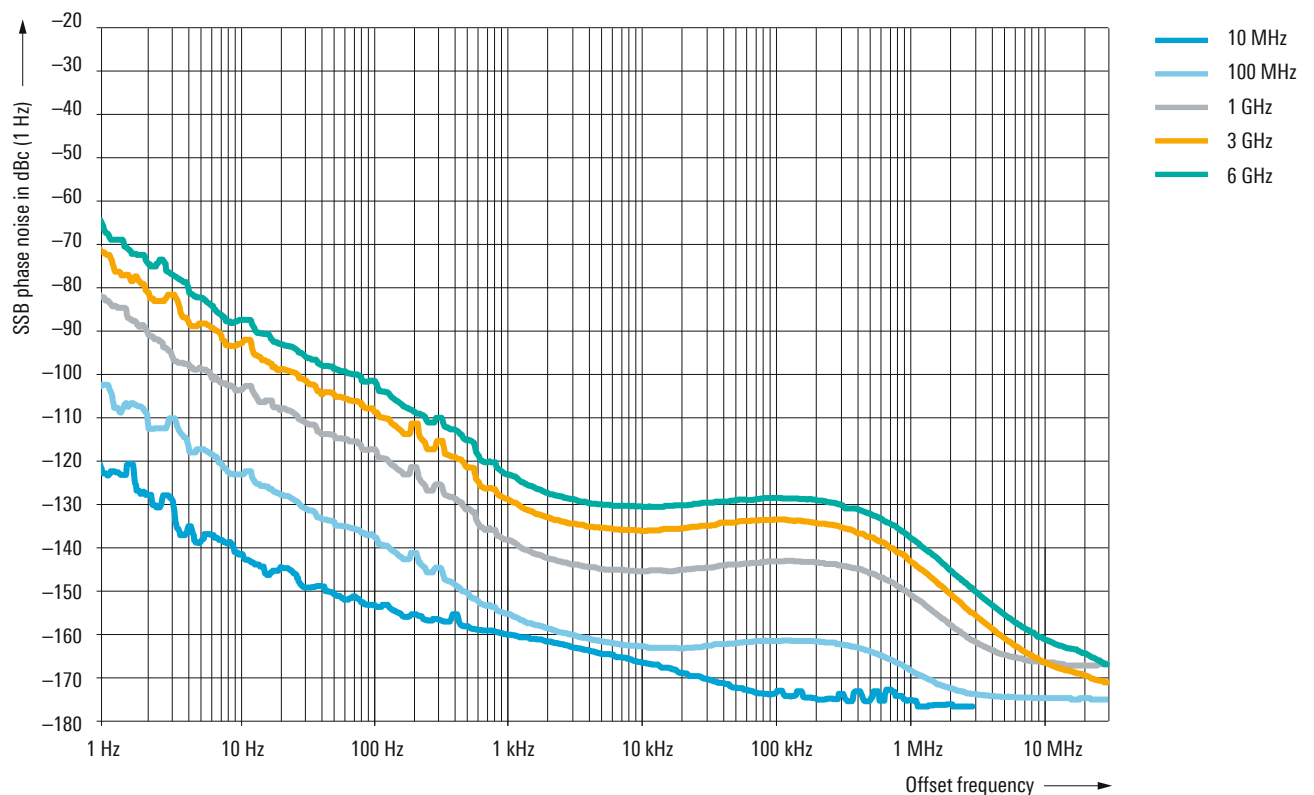
Measured SSB phase noise of clock synthesizer with the R&S®SMAB-B29, R&S®SMAB-B711 and R&S®SMAB-K722 options.
