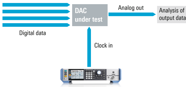
Typical test setup for verifying a DAC.
