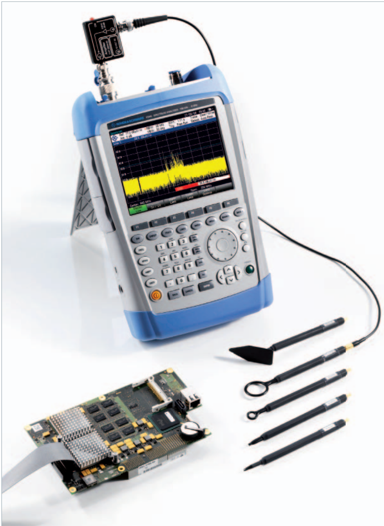
带近场探头的R&S®FSH与待测设备 (DUT)
