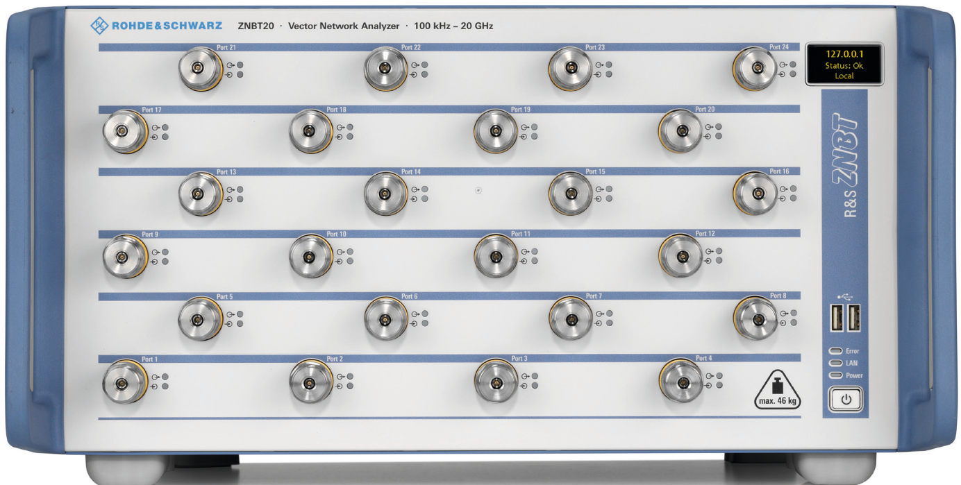
The R&S®ZNBT20 with 24 ports.
